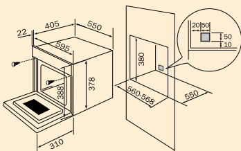
尺寸 (mm) Dimensions (mm)
