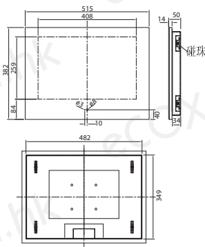
Diagramme for Model: BKW191 (Mirror)
